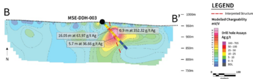
Figure 5: Cross Section looking north on IP chargeability PDP geophysics
