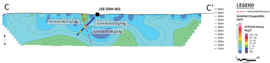
Figure 3: Cross Section looking north on IP chargeability PDP geophysics
