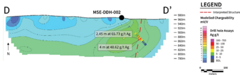
Figure 4: Cross Section looking North on IP chargeability PDP geophysics
