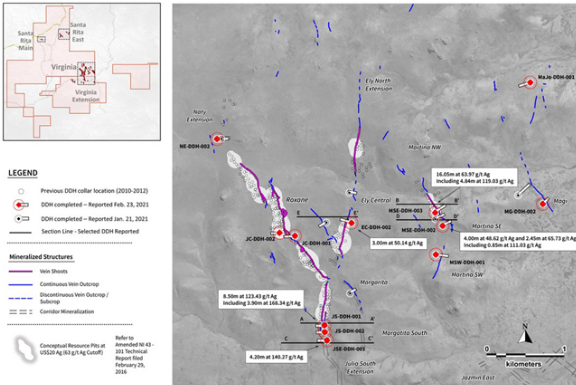
Figure 1: Plan map with the Phase I drill hole locations and conceptual pit shells related to the current resource
