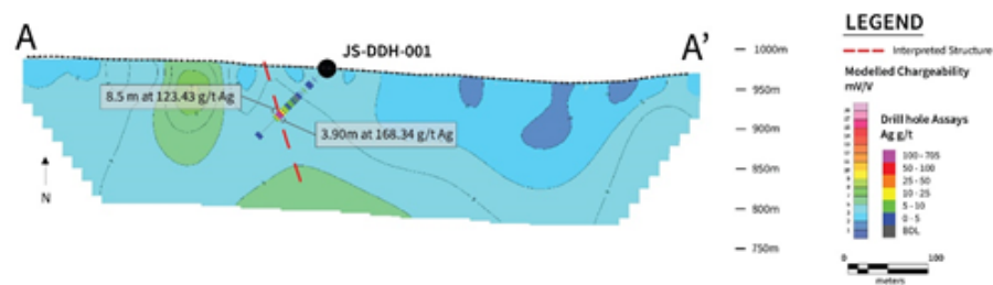
Figure 2: Cross Section looking north on IP chargeability PDP geophysics
